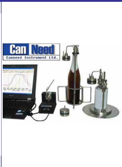
CAN-85B, CAN-125B Pasteurization Temperature Monitor (PU Monitor)
